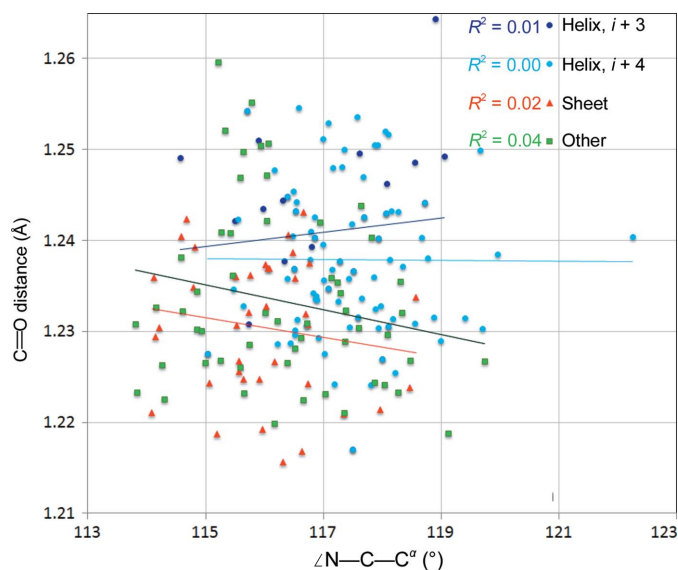
Figure 18 Scatterplot of the C=O distances versus the \angle C^{\alpha}-C-N angles. The linear fits are shown to highlight the average values of distances (despite correlation coefficients of close to zero between the two variables).
